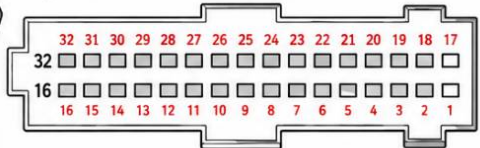
T32 pinout (view from rear, wiring side)
