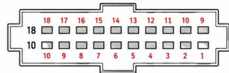
T18 pinout (view from rear, wiring side)
